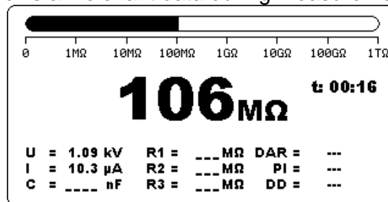
Figure 3.7: Measurement window
